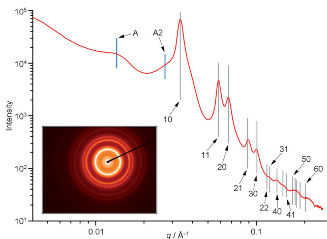
Figure 2. Transmission SAXS pattern recorded on a 100 \mu\text{m} \times 250 \mu\text{m} section. Gray lines indicate the positions of hcp reflections (labels are Miller indices (hk) for the reflections; not all are shown for clarity). The inset shows the associated diffraction pattern.
