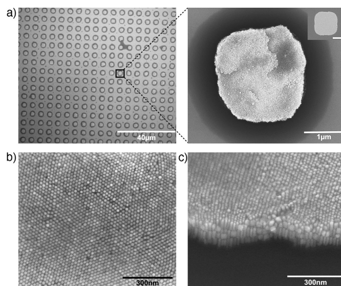
Figure 1. SEM images of self-assembled standing arrays of GNRs on a micropatterned substrate grown from a 9 nm solution at a temperature of 45 °C. a) Low-magnification image of GNR arrays and a close-up image of one individual pattern after self-assembly. The inset shows one micropattern before assembly. b) High-resolution SEM image of a GNR array. c) SEM image recorded at a tilt angle of 52°.
